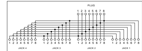
LABEL DETAIL AND WIRING DIAGRAM
